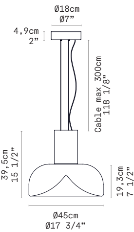
AELLA S 45 L
