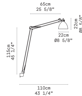
JJ MID - WALL
