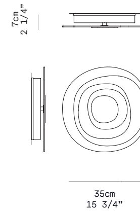
BETA SMALL P-PL
