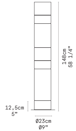
STACKING TR D
