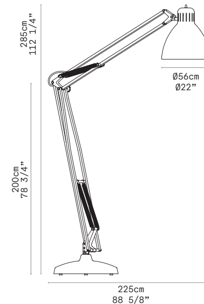
JJ GREAT - FLOOR
