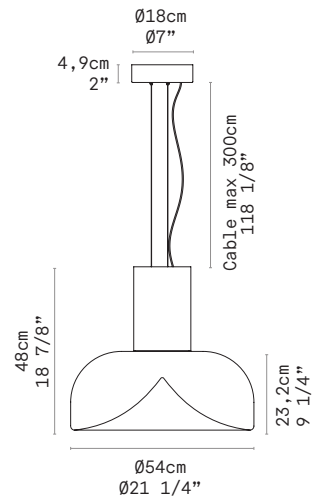
AELLA S 54 L
